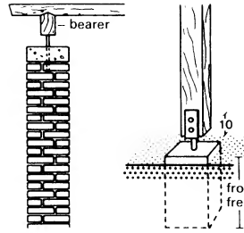
2 Pergola on brick pier 3 Raised timber frame (avoids rot)
